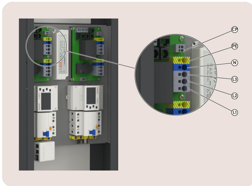
Image 11: View on the cable connections
